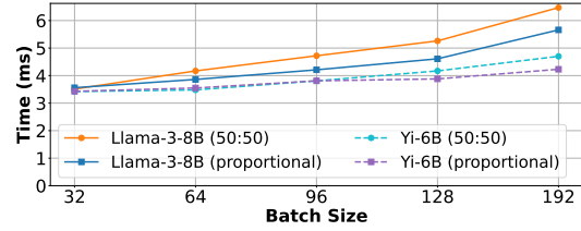
Figure 14. Effect of scheduling policy in POD-ATTENTION.
