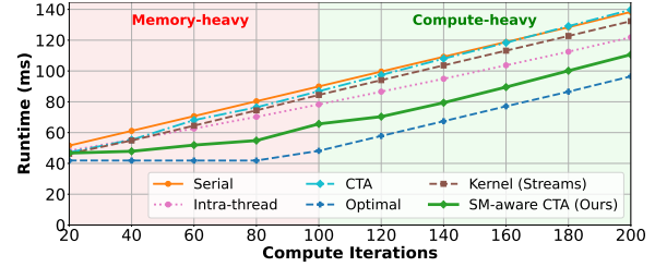
Figure 7. Fine-grained fusion versus serial computation.
