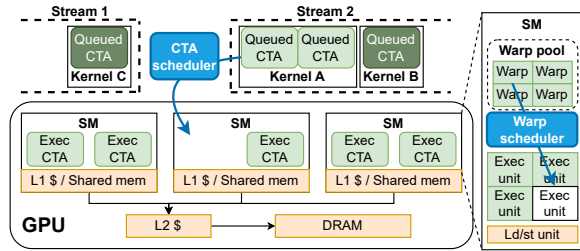
Figure 5. GPU execution model.
